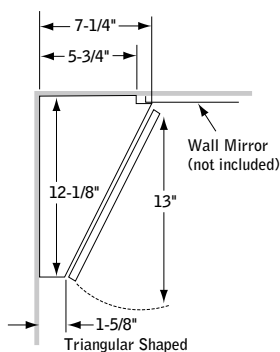
Top-down view of left hand Avanti 631 Corner Cabinet as shown in photo above.
